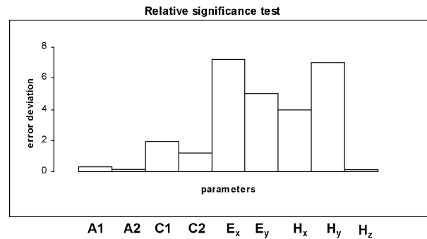
Figure 9. Relative significance of various inputs to the networks, namely amplitude ratios (A1 and A2), correlation coefficients (C1 and C2) and five-pattern qualities ( E_x , E_y , H_x , H_y and H_z ). The error deviation against each input is a measure of its significance to the neural network.
